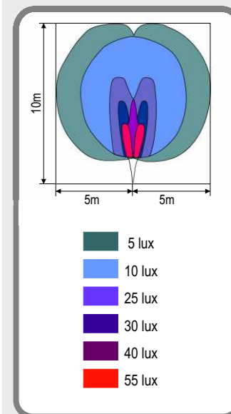
Isolux diagram
