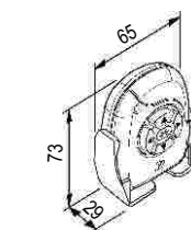
Remote Control Head
