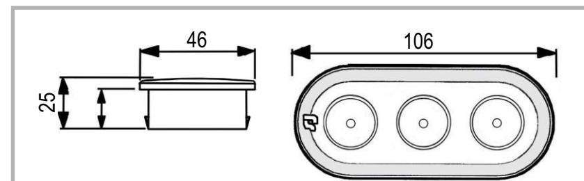
A Microled Advance méretei (mm)
